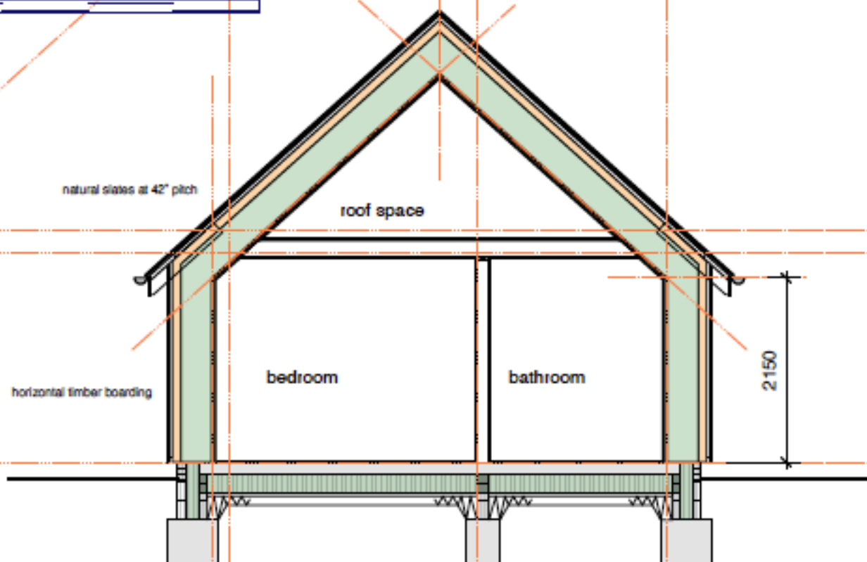
SECTION THROUGH BEDROOM 1
