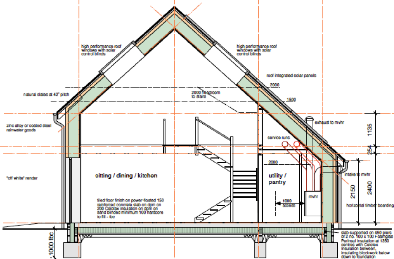
SECTION at STAIRS
