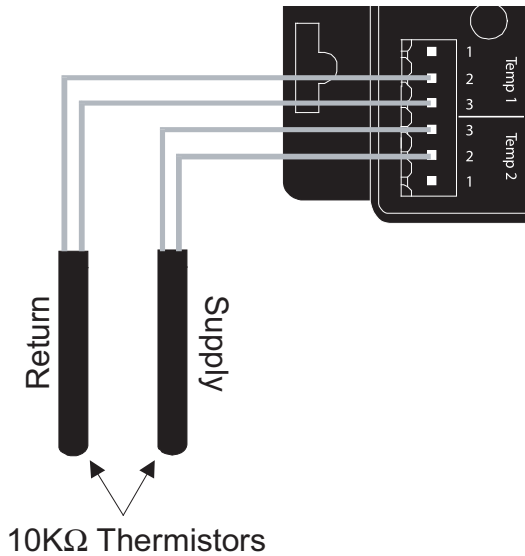
Thermistor Wiring Diagram
