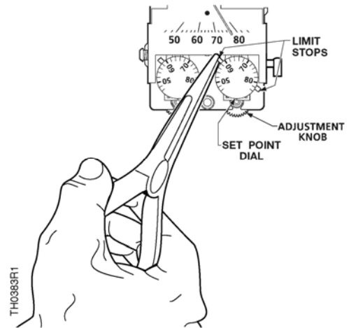
Figure 8. TH 192 DN and DNV Limit Stop Adjustments.
