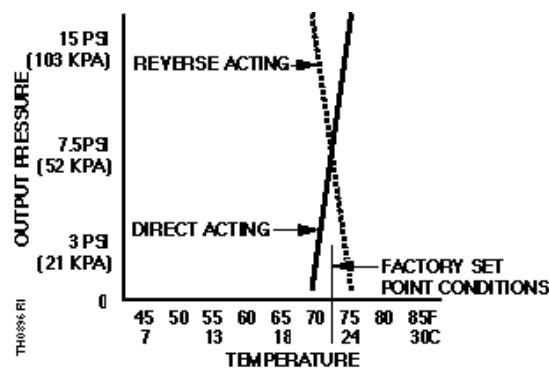
Figure 5. TH 192 DN and DNV Input/Output Characteristics.
