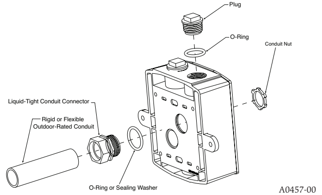
FIGURE 5: LIQUID-TIGHT CONNECTORS
