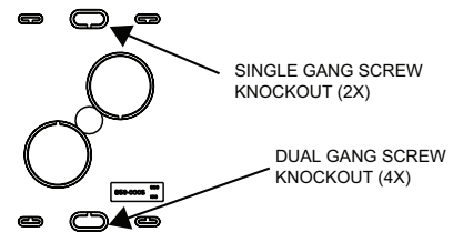
FIGURE 4. SCREW KNOCKOUT REMOVAL WITH SCREWDRIVER:
