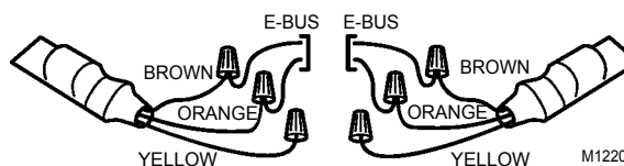
Fig. 5. Physical connection of modules for a double termination network .
