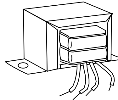
UL1015#18 LENGTH 8" IN COLOR "WHITE", "BLACK", "RED" & " ORANGE"
