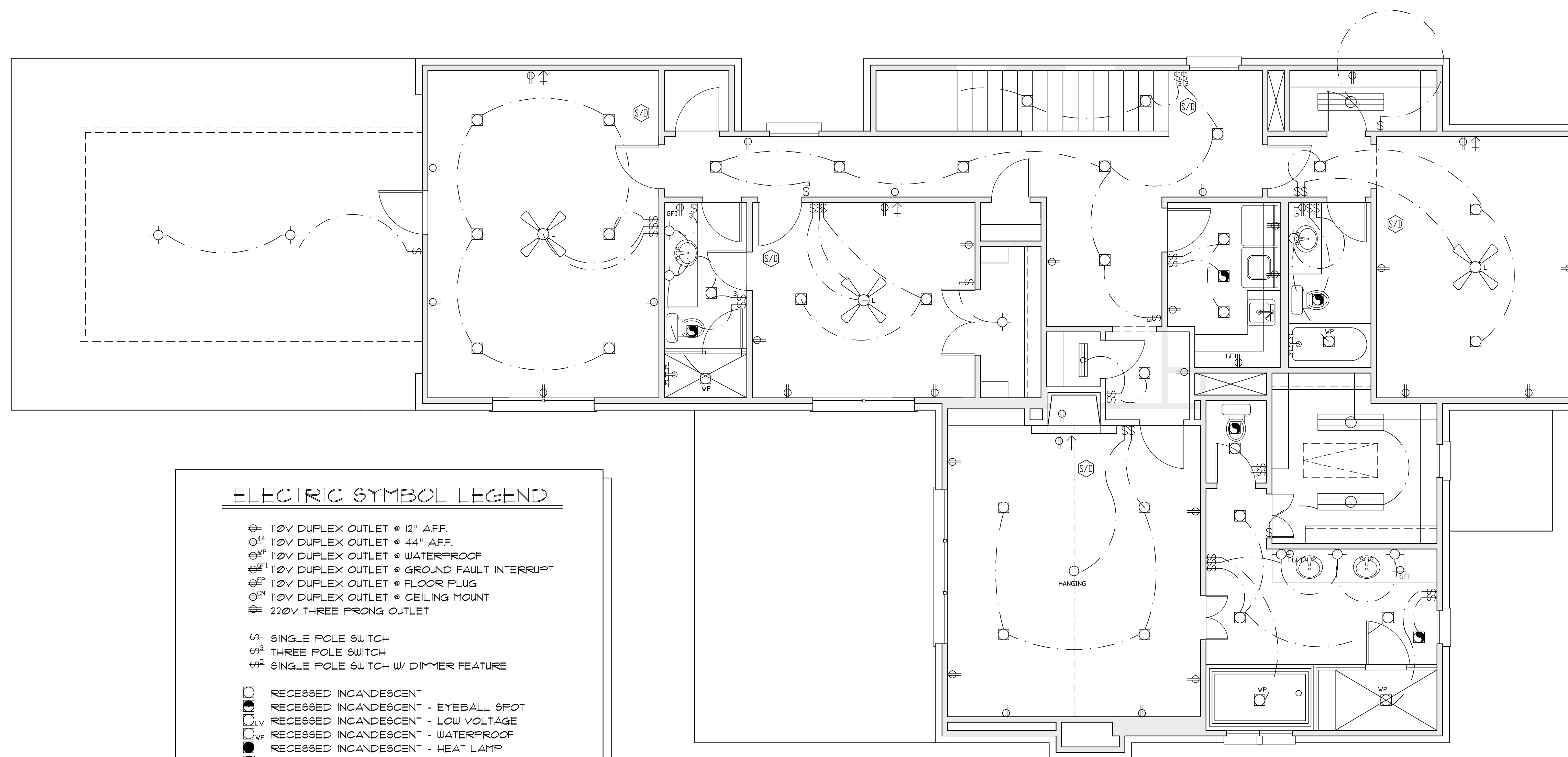
① SECOND FLOOR ELECTRICAL PLAN SCALE: 1/4"=1'-0"
