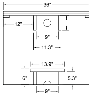
Discreet Wire Cutout on Inside Base Panel
