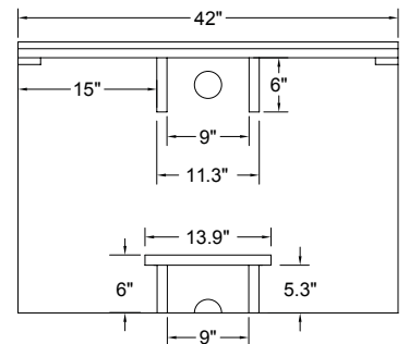
Discreet Wire Cutout on Outside Base Panel
