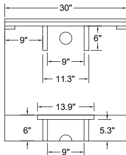
Discreet Wire Cutout on Outside Base Panel
