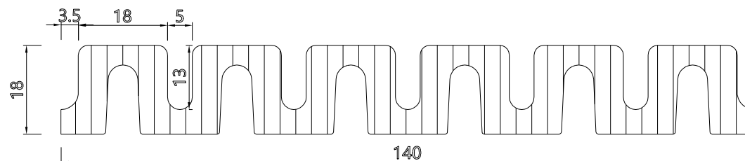
FRONT SCALE 1/1
