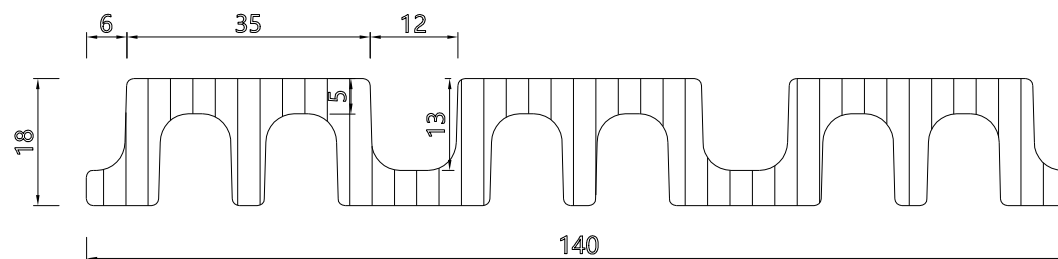
FRONT SCALE 1/1
