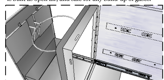
Right side Multi-Drawer has Built-in Trash Bag Ring, for an easy solution for cluttered spaces, or secure tank in place.
