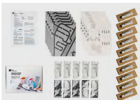
Bare Conductive Electric Paint Circuit Pack SKU: 197-6852 MPN: SKU-1527
