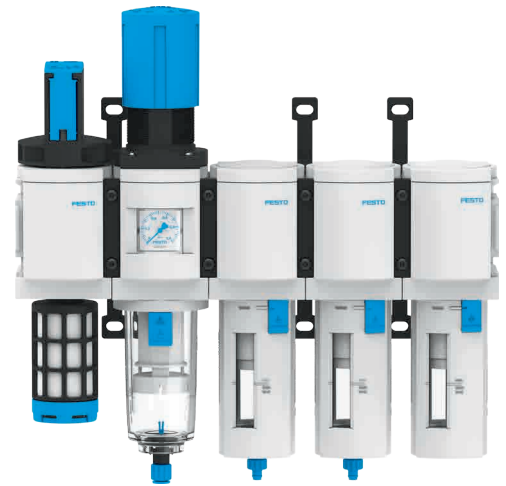
Fig. 3: Example – Festo service unit MSB6
