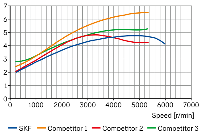
Friction [Nm]
