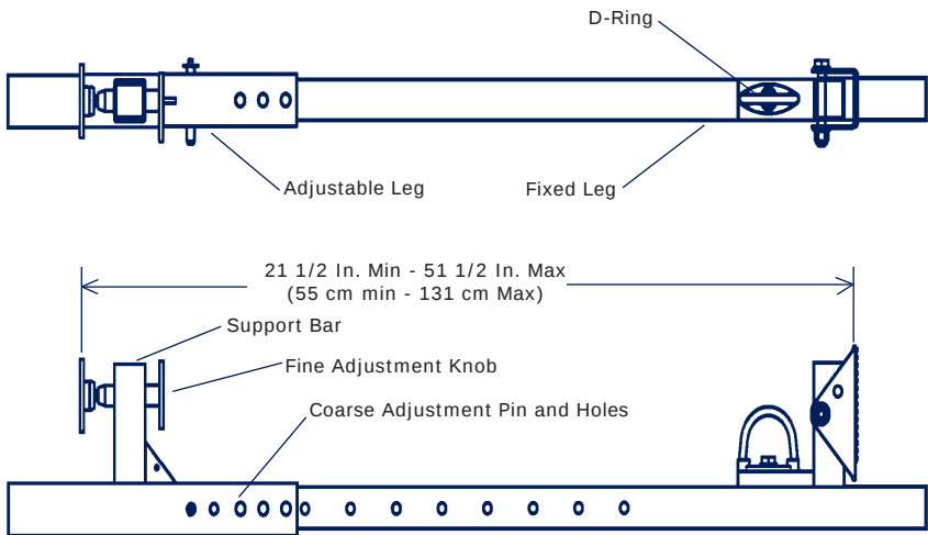
Figure 1 - Door Jamb Anchor
