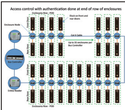
Access control with authentication done at end of row of cabinet
