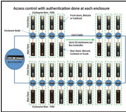
Access control with authentication done at each cabinet
