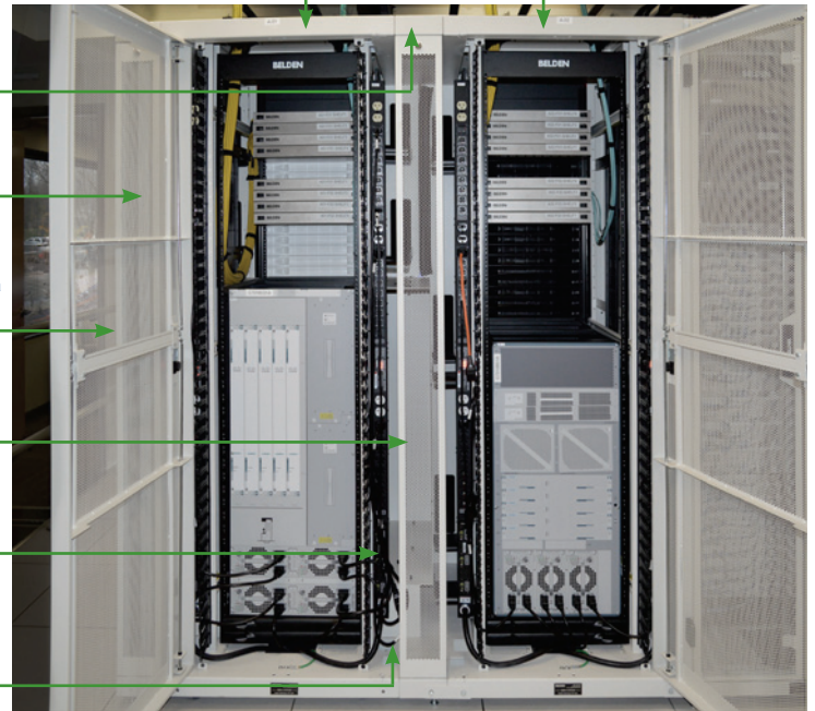
Ganged XN frames with end-of-row 6" extension and between cabinet 6" extension (rear view)
