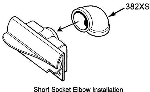
Short Socket Elbow Installation
