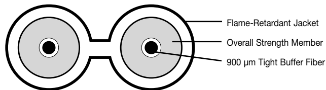
Duplex Zipcord
