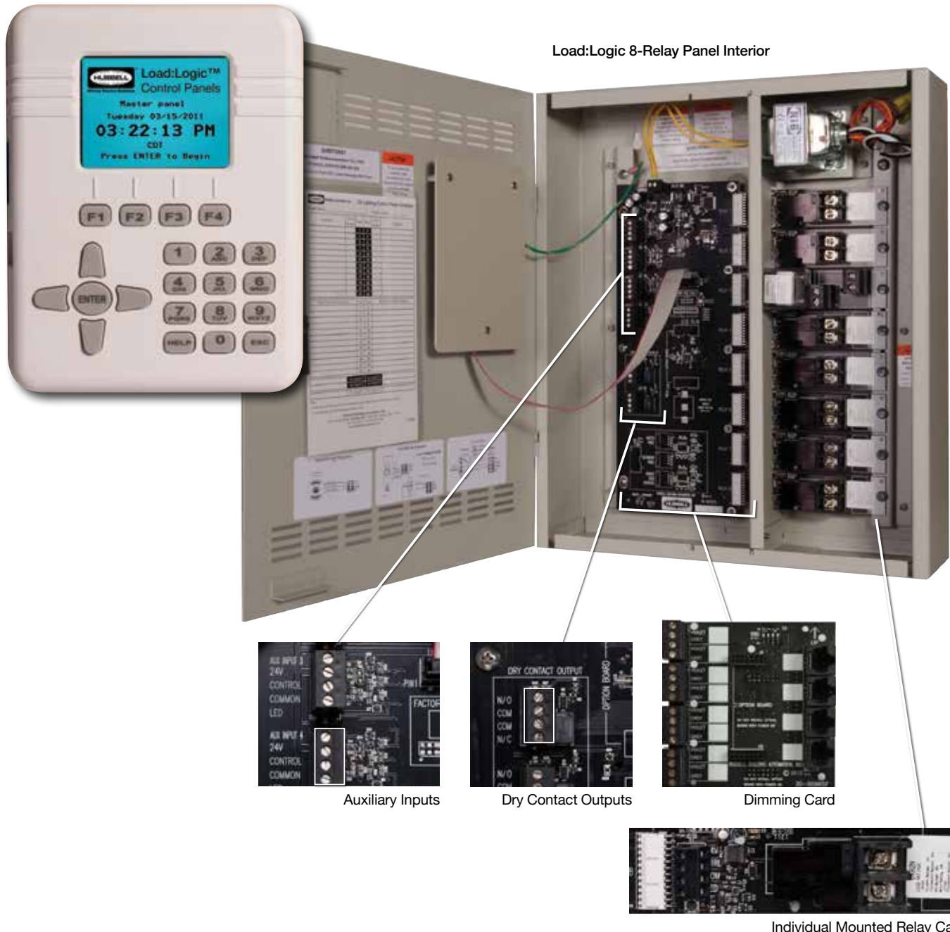
Individual Mounted Relay Card
