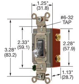
HBL1221ILC
