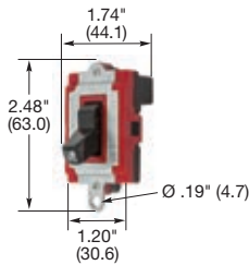
SNAPSWJUMP
