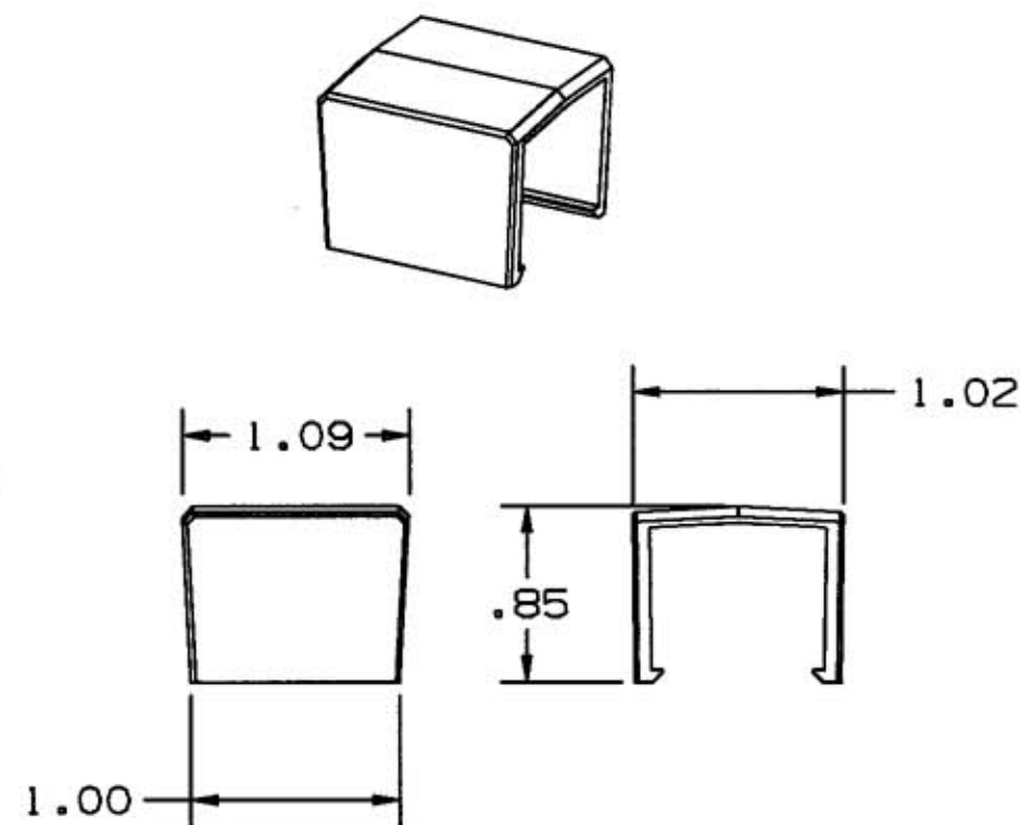
SPLICE COVER
