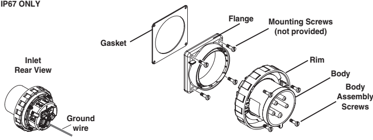
FIGURE 5: 63A & 125A INLET IP67 ONLY
