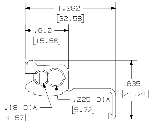
TERMINATION CLIP
