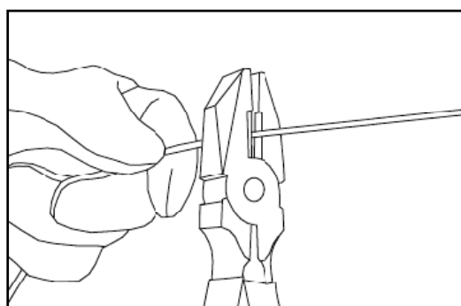
Exposing the central strength member
