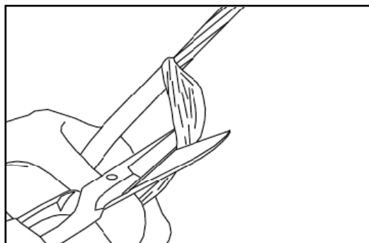
Removing the split cable sheath
