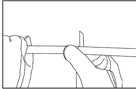
Ring the cable sheath with a sheath knife
