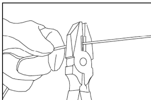
Cutting the central strength member
