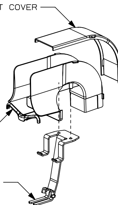
SUPPORT BRACKET
