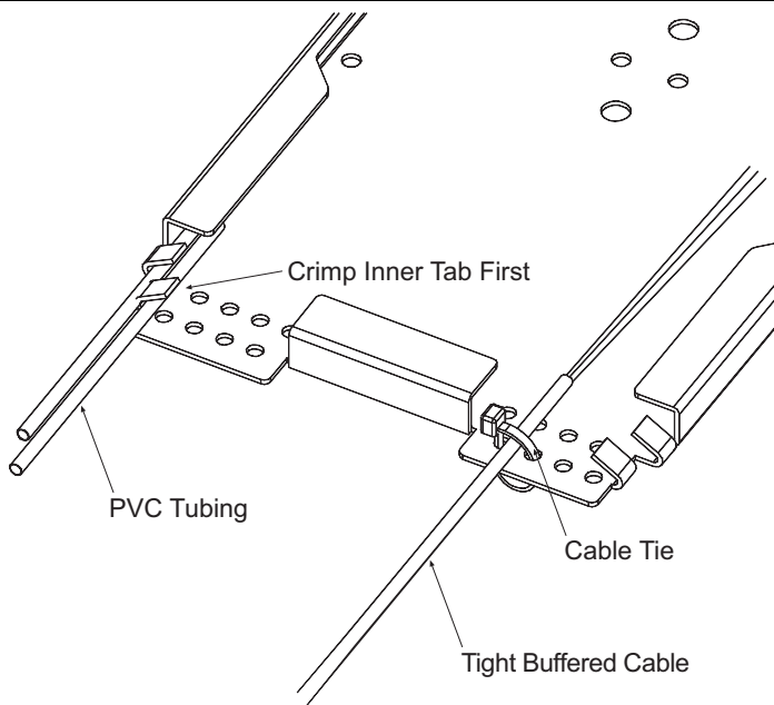
Buffered Fiber
