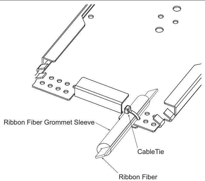
Ribbon Fiber
