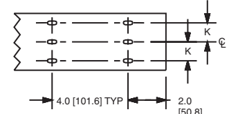
Type H 2", 3", and 4" wide duct.
