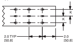
Type HN 2", 3" and 4" wide duct.
