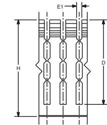
Type HN: Multiple slot restrictors present with 3" and greater duct wall height.
