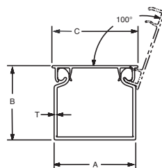
Type HN: Multiple slot restrictors present with 3" and greater duct wall height.
