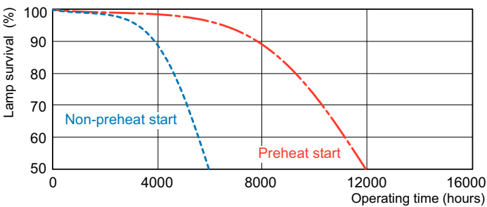
MASTER TL5 Circular Life Expectancy 3 h cycle
