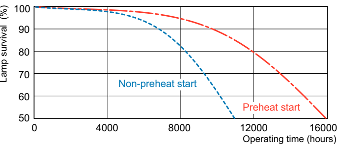
MASTER TL5 Circular Life Expectancy 12 h cycle
