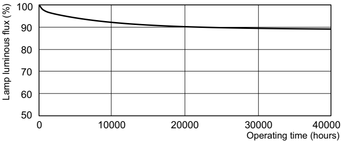
MASTER TL5 HO EcoPlus Lumen Maintenance 3 h + 12 h cycle
