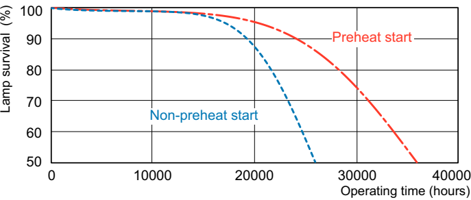
MASTER TL5 HO EcoPlus Life Expectancy 12 h cycle
