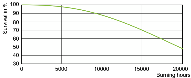
Life Expectancy Diagram - MHC100/U/MP/3K ELITE
