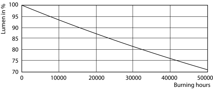
Lumen Maintenance Diagram - 8.5PL-C/T/COR/26H-835/IF9/P/4P/DIM 10/1
