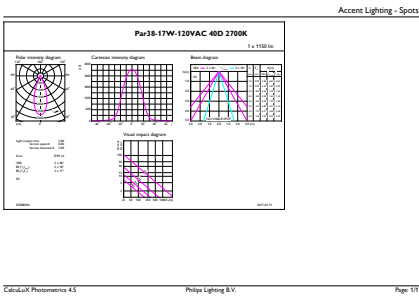
Accent Lighting Spots - 17PAR38/EXPERTCOLOR/F40/927/DIM
