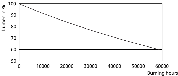
Lumen Maintenance Diagram - 12PAR30L/EXPERTCOLOR RETAIL/ F40/930/DIM
