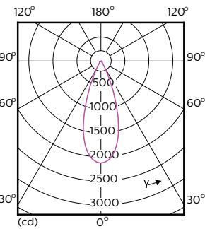
Light Distribution Diagram - 12PAR30L/EXPERTCOLOR RETAIL/F40/930/DIM
