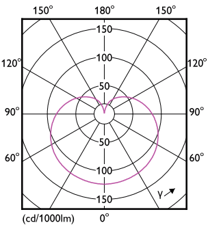
Light Distribution Diagram - 8.8A19/PER/927-22/P/E26/WG 6/1FB T20
