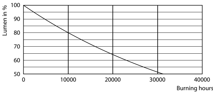
Lumen Maintenance Diagram - 8.8A19/PER/927-22/P/E26/WG 6/1FB T20
