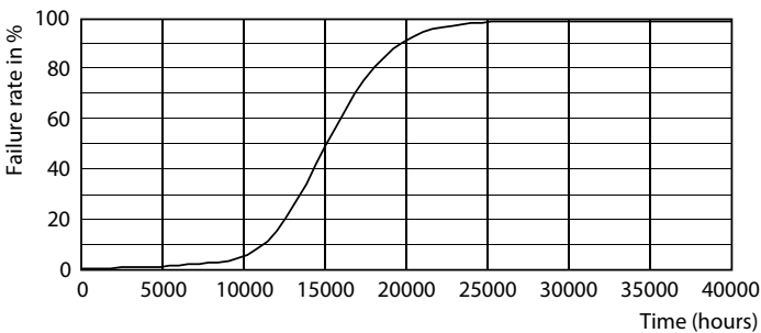
Life Expectancy Diagram - 8.8A19/PER/927-22/P/E26/WG 6/1FB T20
