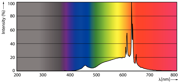
Spectral Power Distribution Colour - 8.8A19/PER/927-22/P/E26/WG 6/1FB T20
