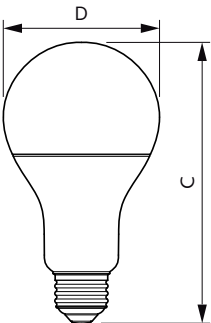
Bulb A21 16-100W 1600lm 2200-2700K E26
