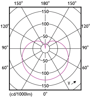
Light Distribution Diagram - 8.8A19/PER/927/P/E26/DIM 6/1FB T20
