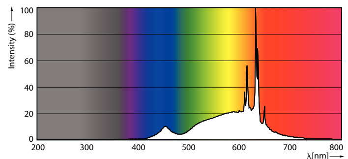
Spectral Power Distribution Colour - 8.8A19/PER/927/P/E26/DIM 6/1FB T20
