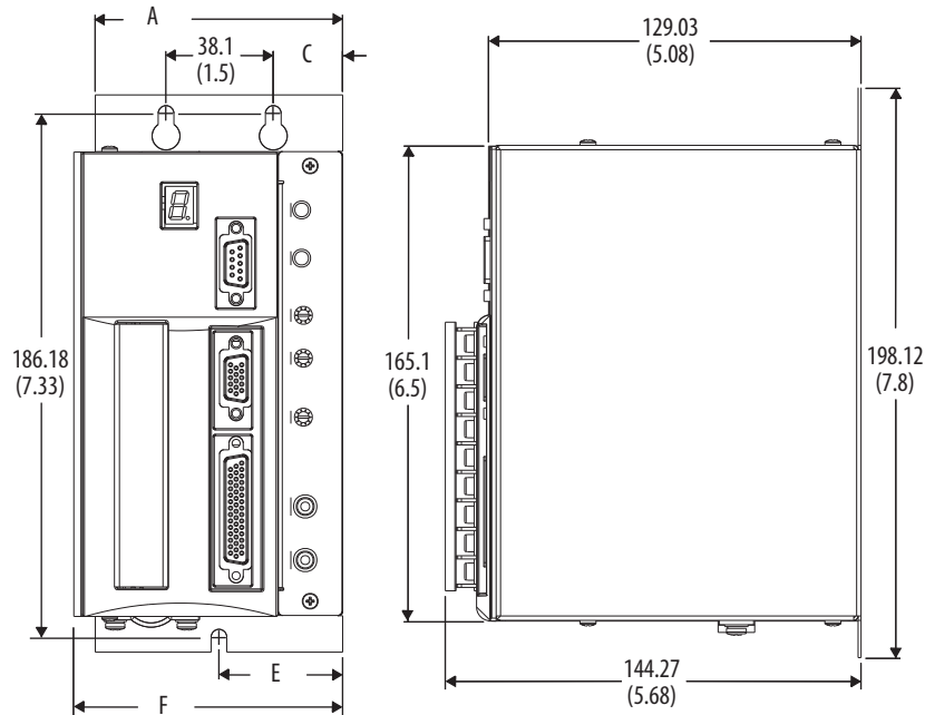
2098-DSD-xxx, 2098-DSD-xxxX, 2098-DSD-xxx-SE, 2098-DSD-xxx-DN, 2098-DSD-xxxX-DN Dimensions
