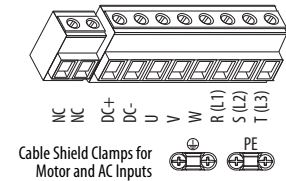
Power Terminal Block 2099-BM09-S
