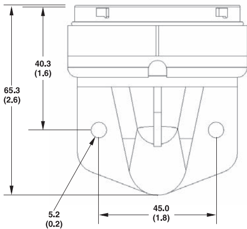
Vertical Mount Base
