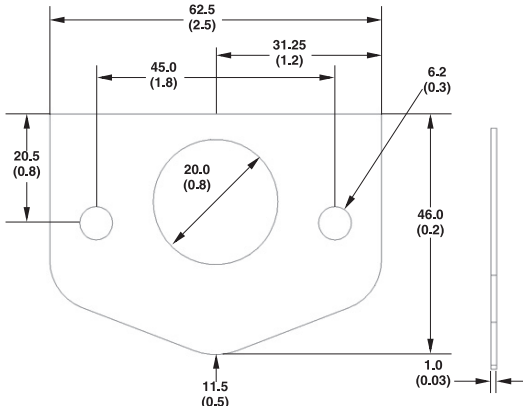
Magnetic Pole Connection Box
