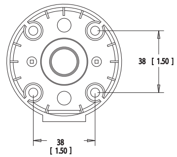
Standard Pole Connection Box
