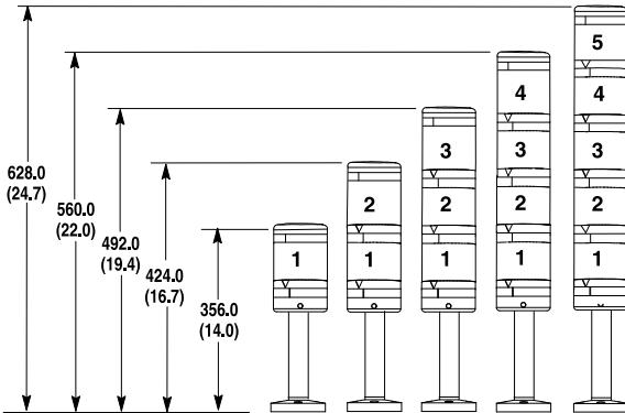
25 cm Pole Mount Base (PM25, SPM25)
