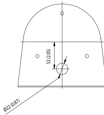
160 mm Beacon, Vertical Bracket
