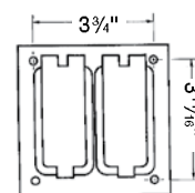
Typical FS mount hole pattern
