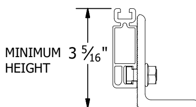
MINIMUM HEIGHT
