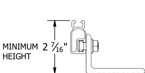
MINIMUM HEIGHT
