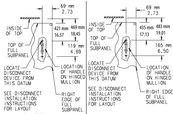
Large Cutout (PROLINE-DD and Type 1 Free-Stand only)
