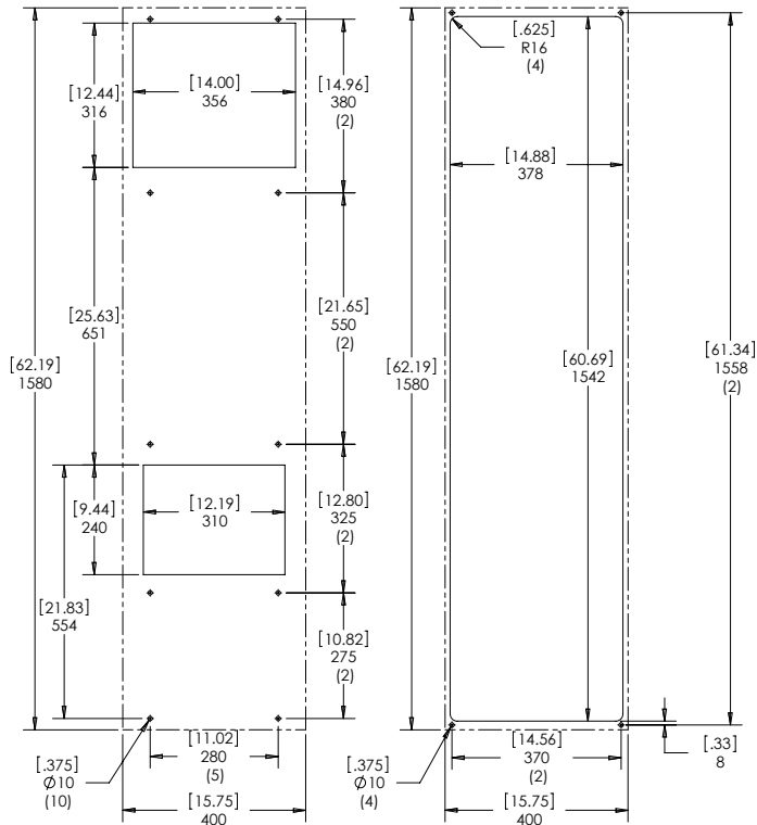
Surface Mount Partial and Full Recess Mount Cutout Dimensions
