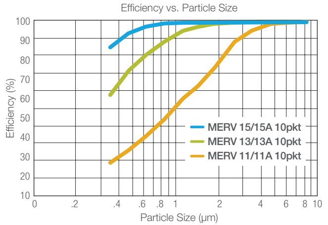
Composite Minimum Efficiency Curve
