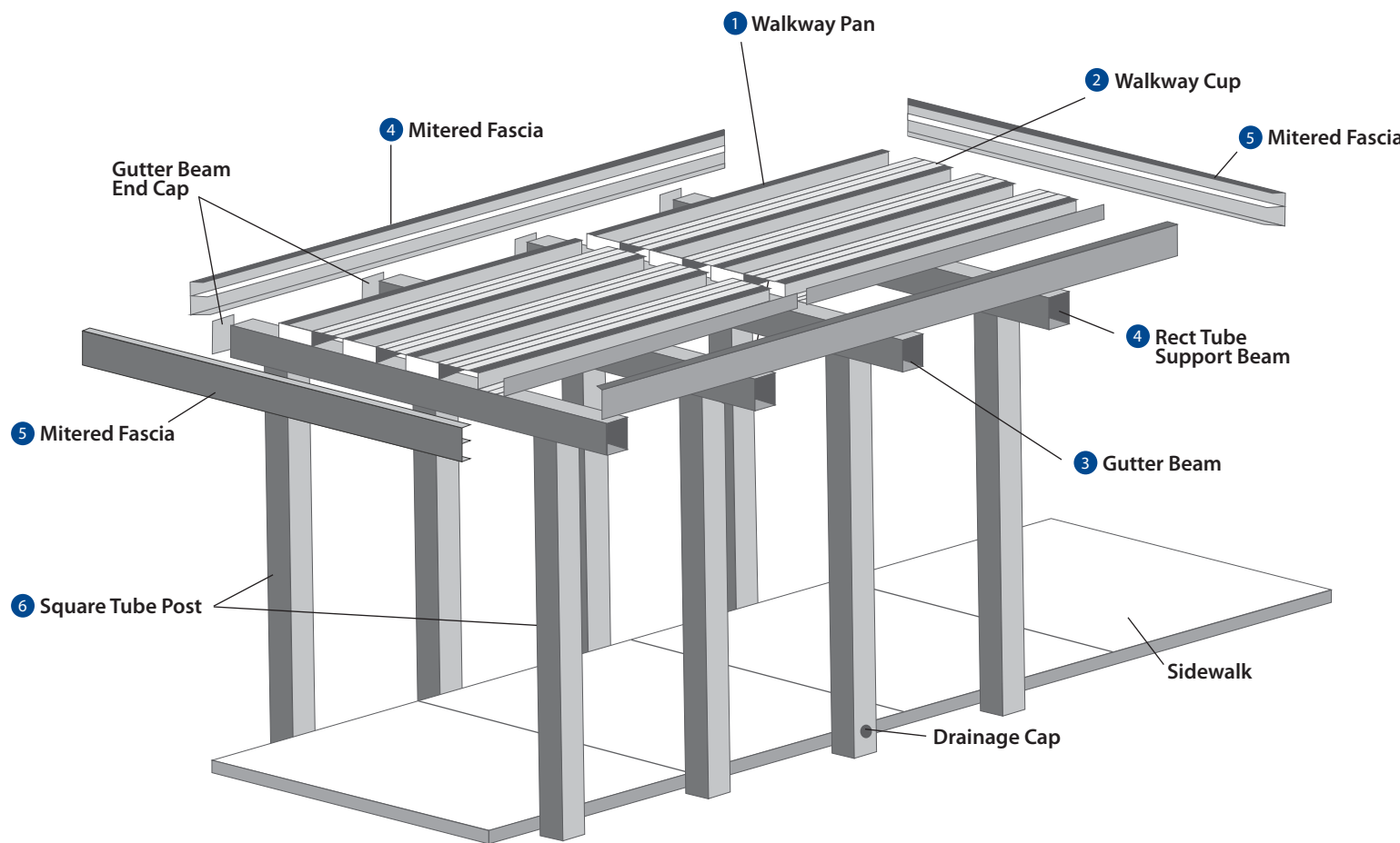
Walkway Pan & Cap Interlocking diagram with relationship to fascia
