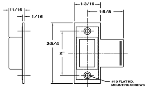
STRIKE PLATE (SHOWN W/DUST BOX)
