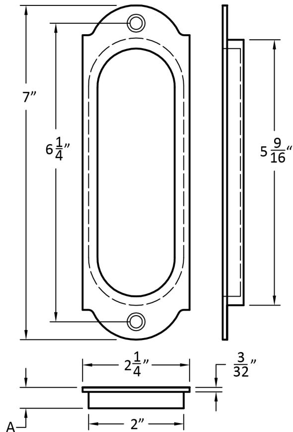
EXPOSED FASTENERS
