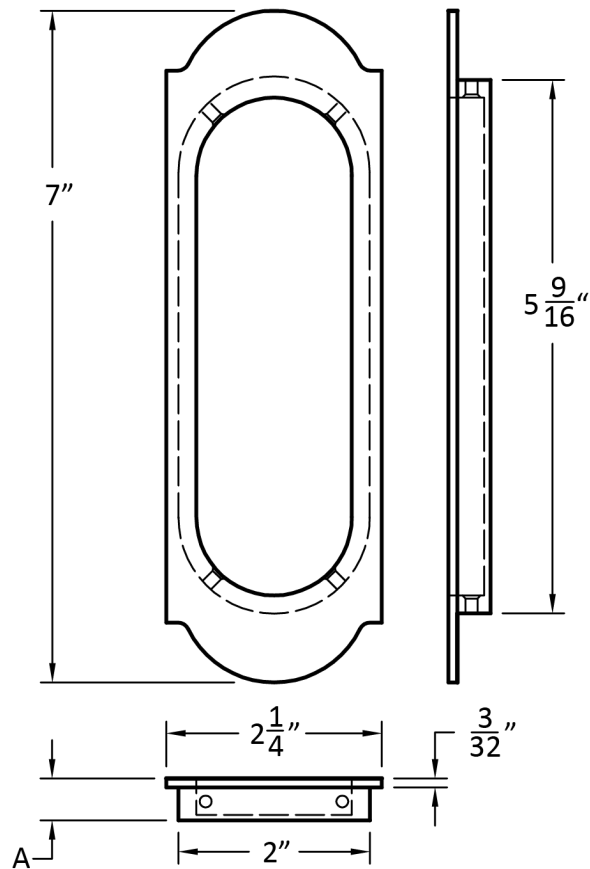
CONCEALED FASTENERS
