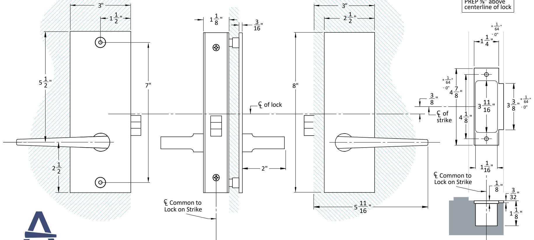
RH Glass Patch with 18L Levers.
