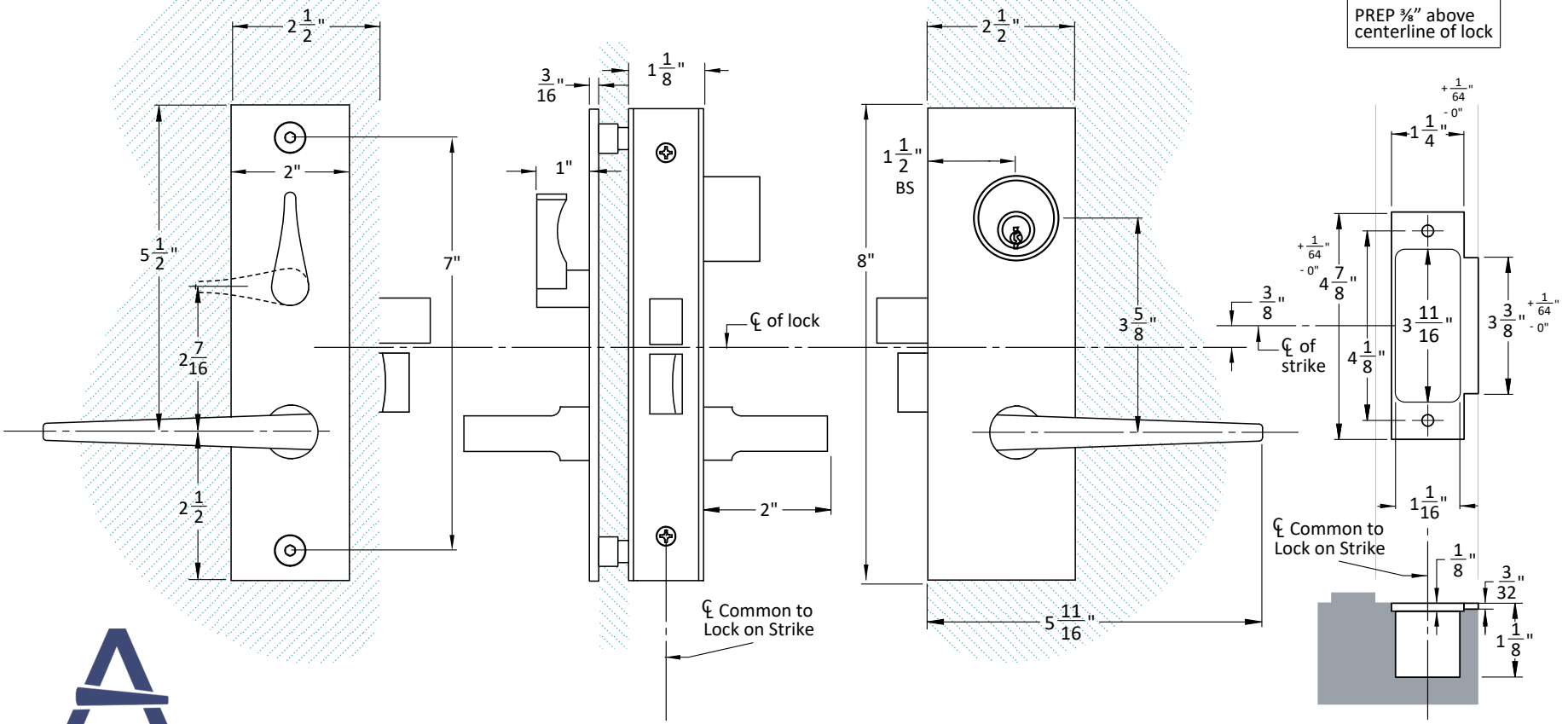
RHR Glass Patch with 18L Levers.
