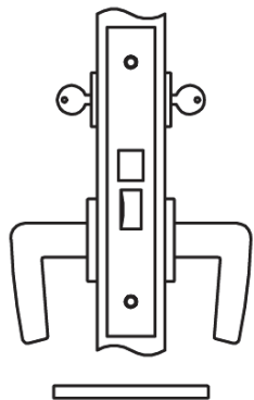
8722UL/8822UL STORE DOOR (ANSI SERIES 1000-F14)
