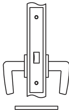
8725UL/8825UL PASSAGE AND CLOSET LATCH (ANSI SERIES 1000-F01)
