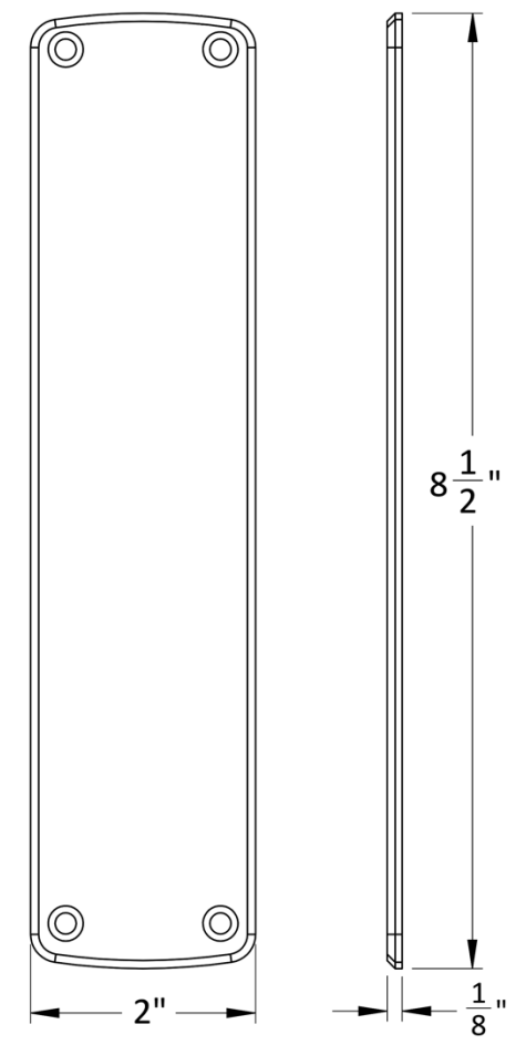
NCP-S-B BLANK PUSH PLATE
