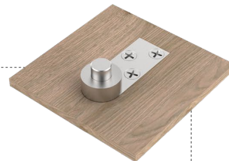
F4 Wood Floor Installation
